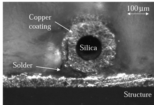
Fig. 1. Copper coated fibre for enhancing temperature sensitivity. The copper has been applied by electrodeposition on a conductively lacquered fibre.
